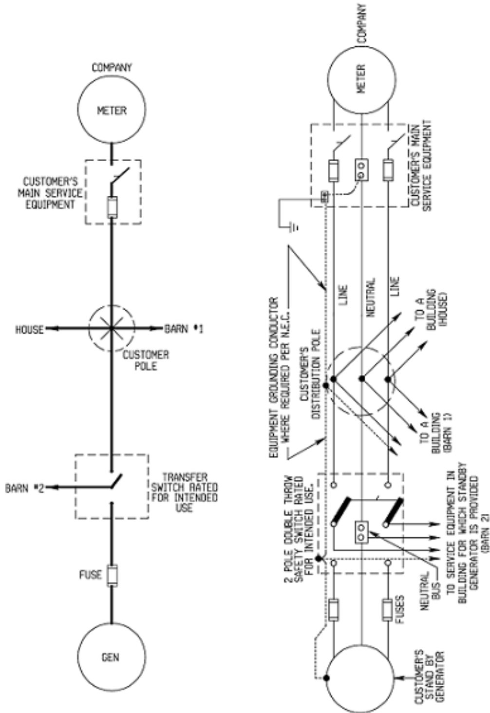
Figure 11.2.1-3 Connection of Standby Generator Supplying One Building from Customer's Main Distribution Point
