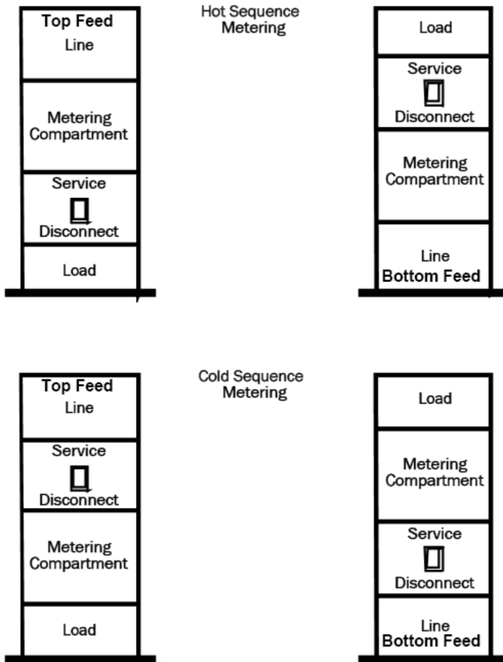
Figure 7.4.6.2-1: Instrument Transformer Metering Sequence - Service Cubicles Rated 600 volts
