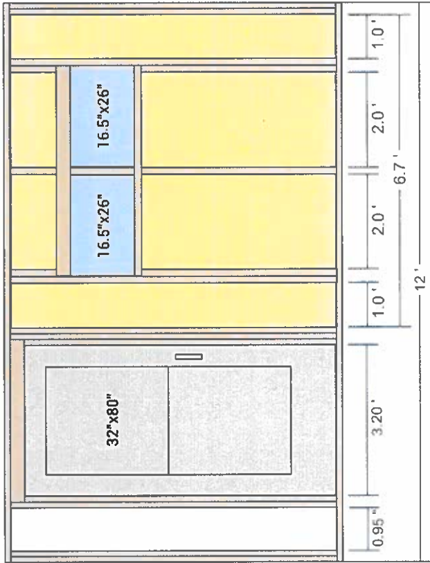
Front Wall
