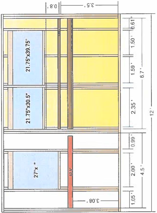
Back Wall
