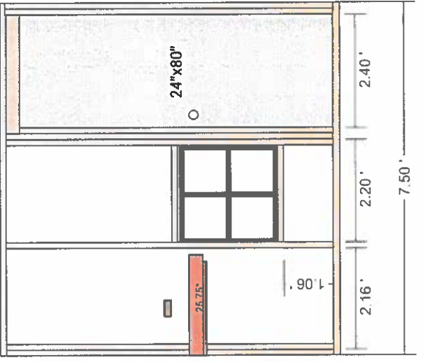
Inner Wall
