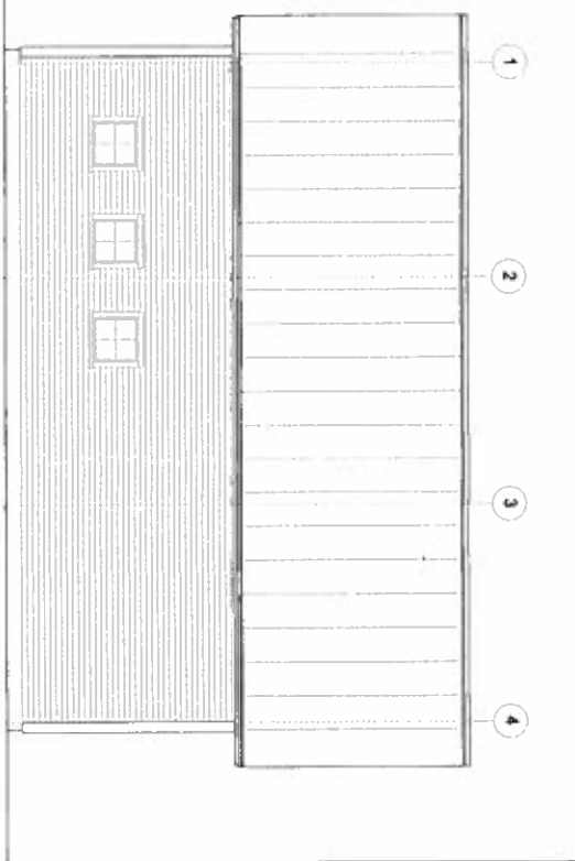
11 SOUTH ELEVATION Scale: 1/4" = 1'-0"
