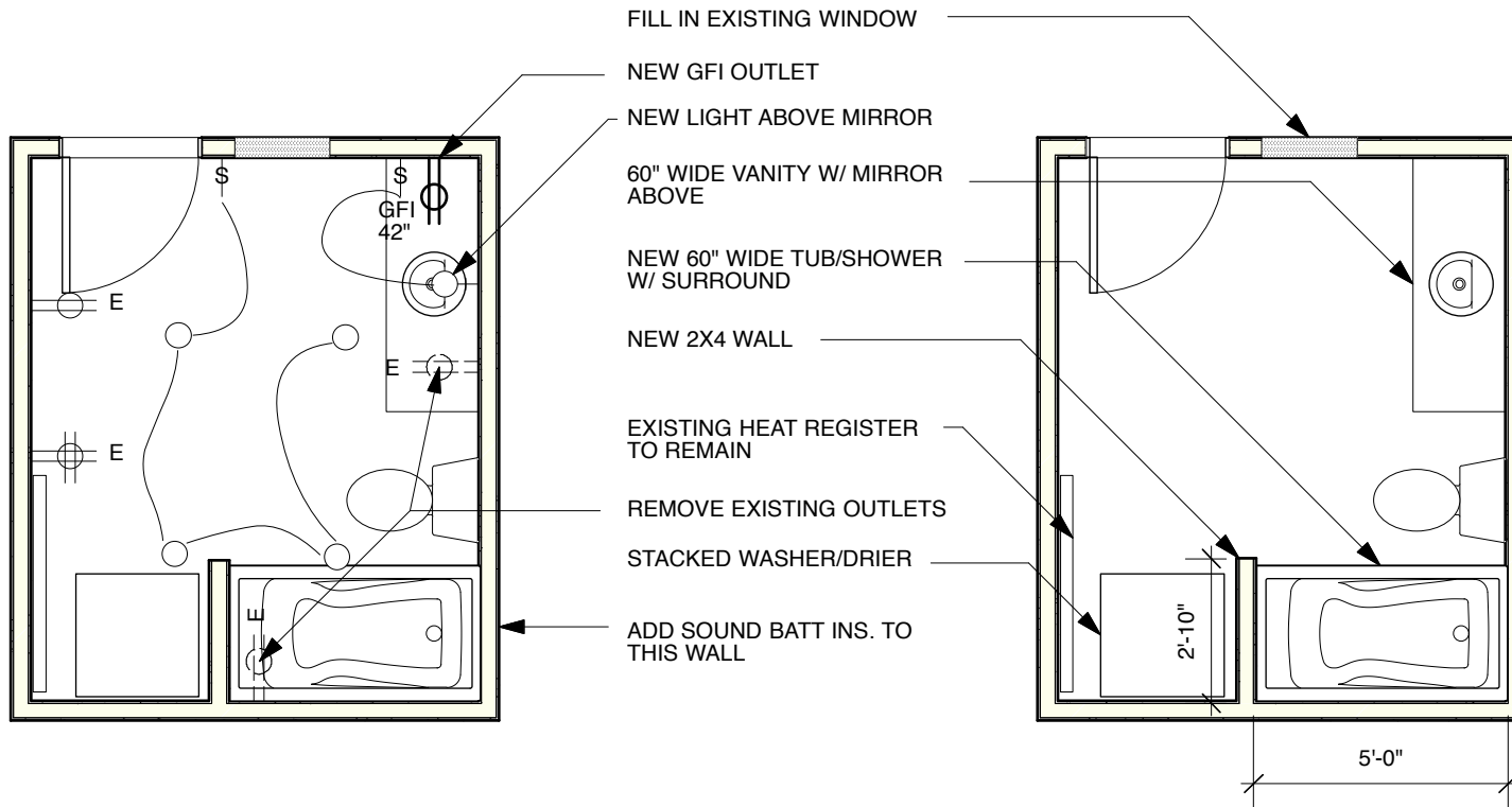
ELECTRICAL PLAN
