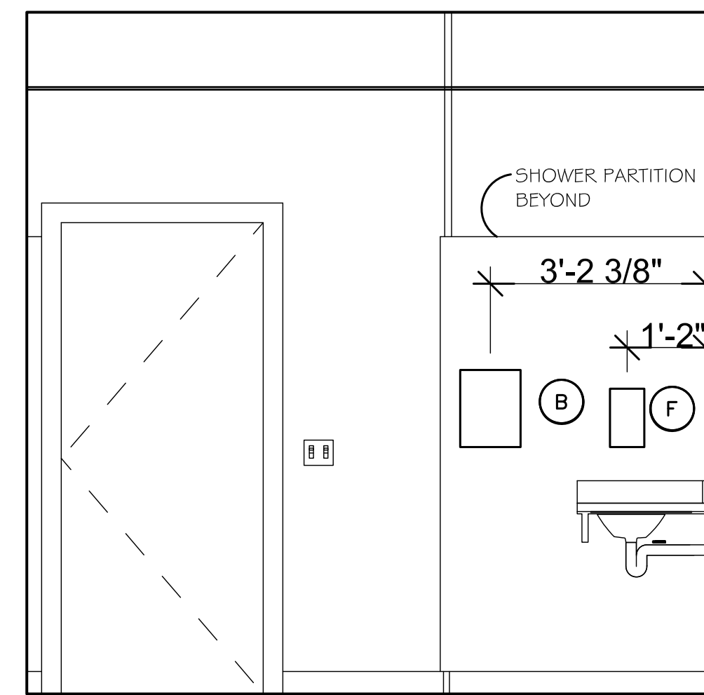
WALL "C"
