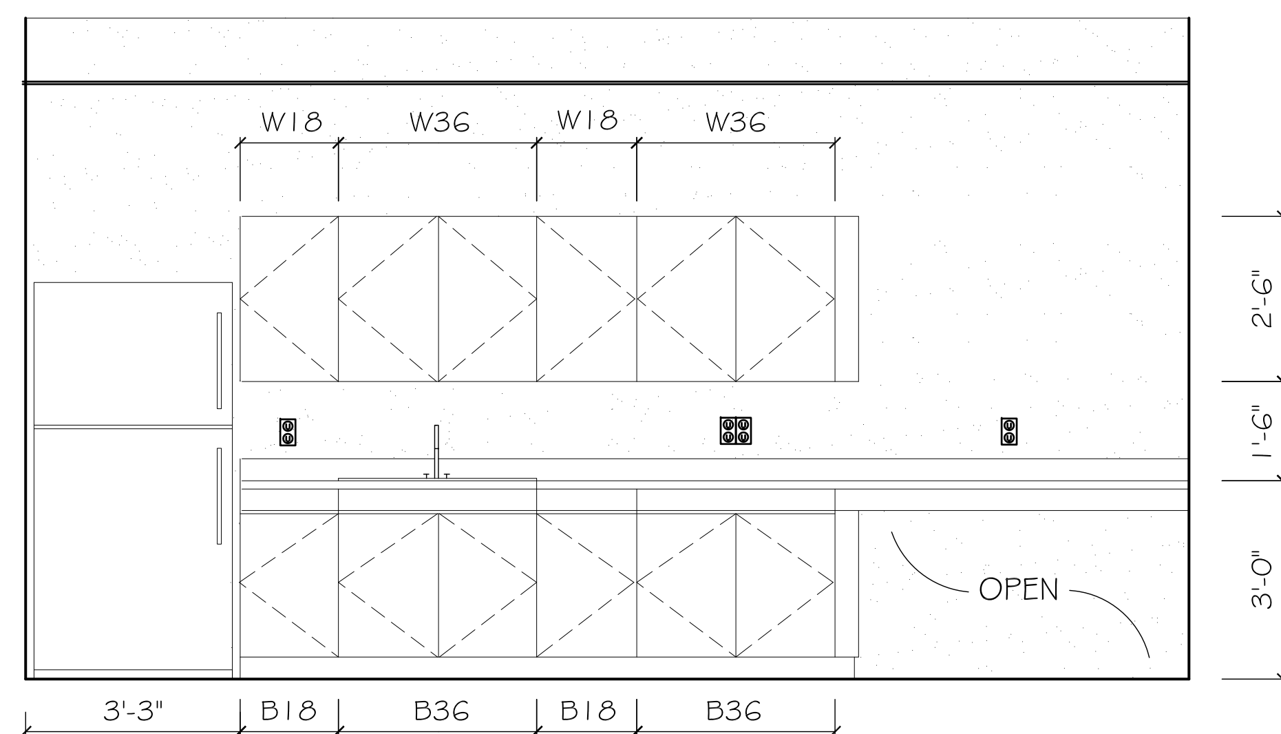
2 INTERIOR ELEVATION BREAKROOM WALL "A" Scale: 1/2" = 1'-0"
