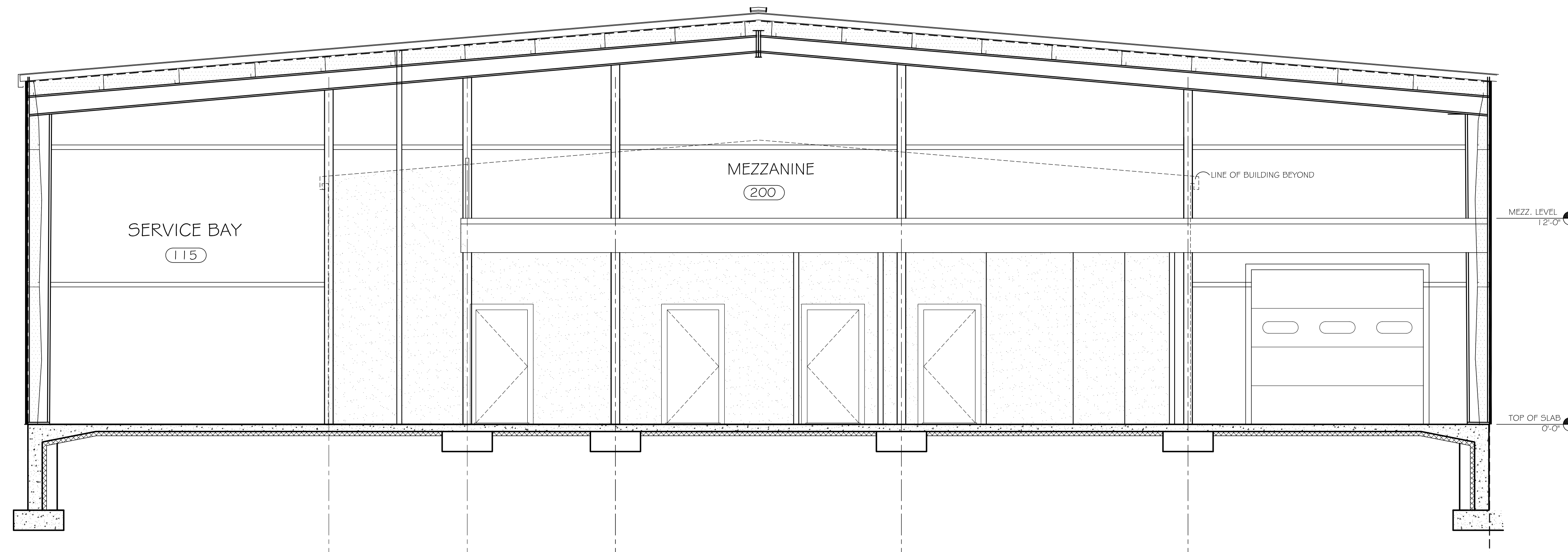
3 BUILDING SECTION "C" Scale: 1/4" = 1'-0"
