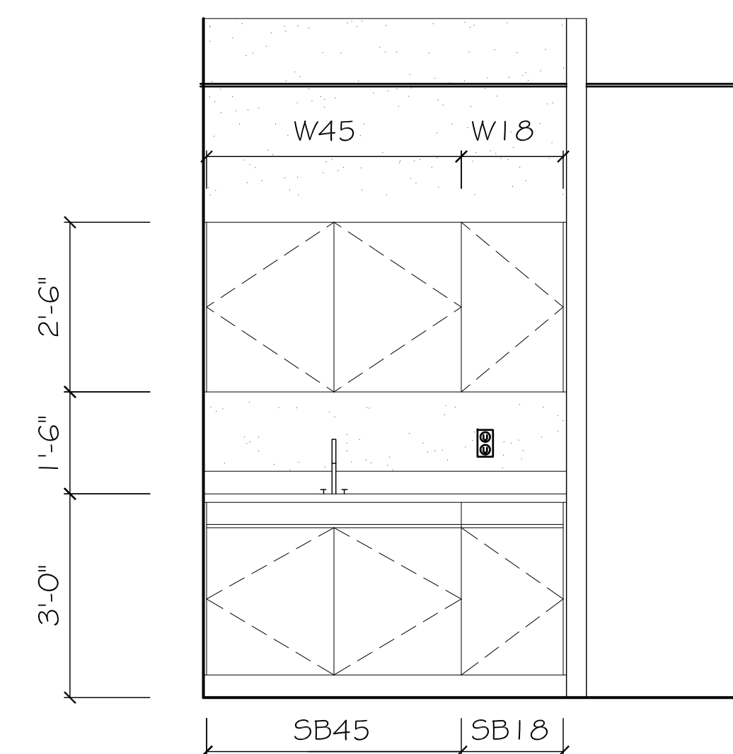
3 INTERIOR ELEVATION HOUSEKEEPING SUPPLIES WALL "A" Scale: 1/2" = 1'-0"
