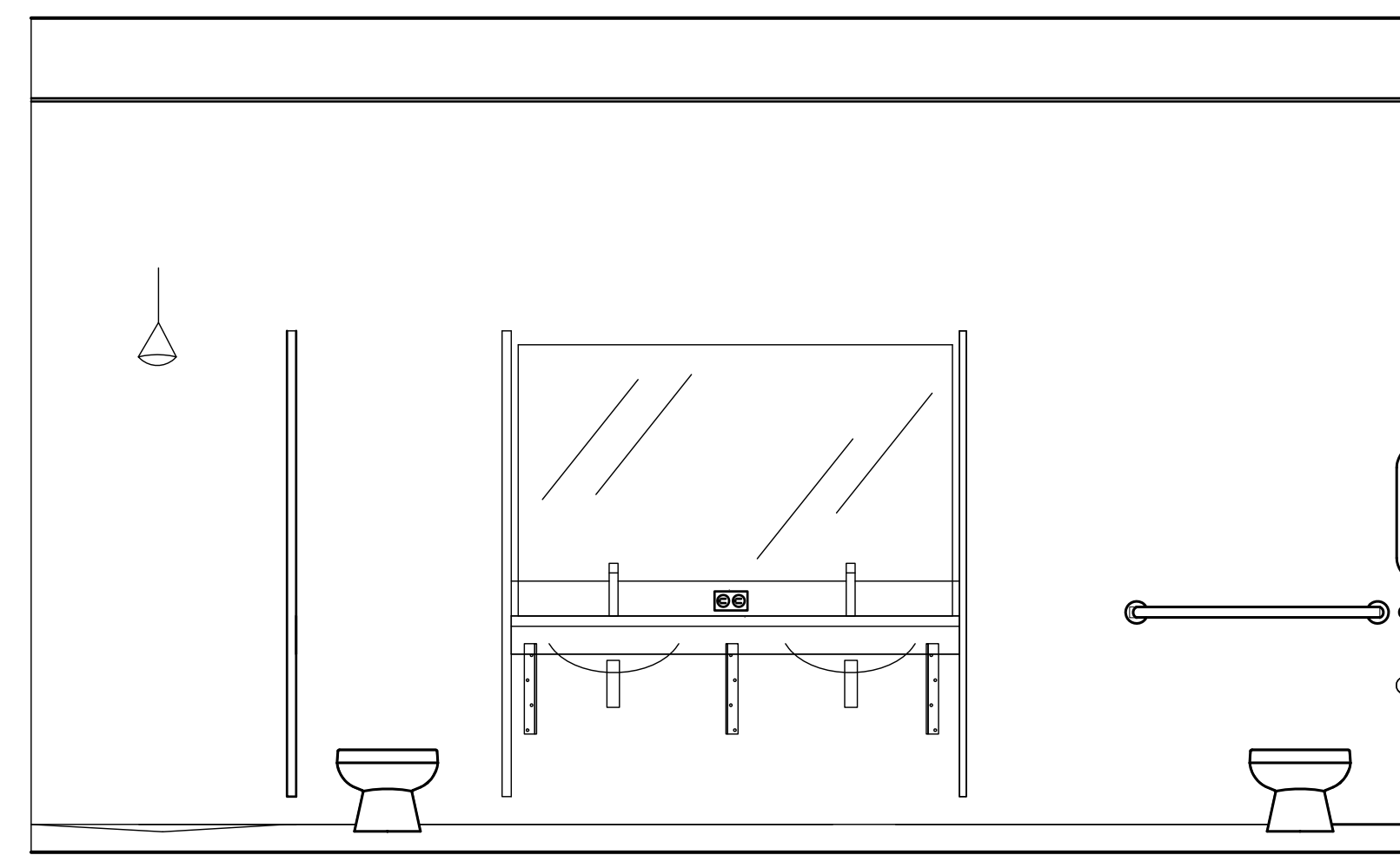
WALL "B"
