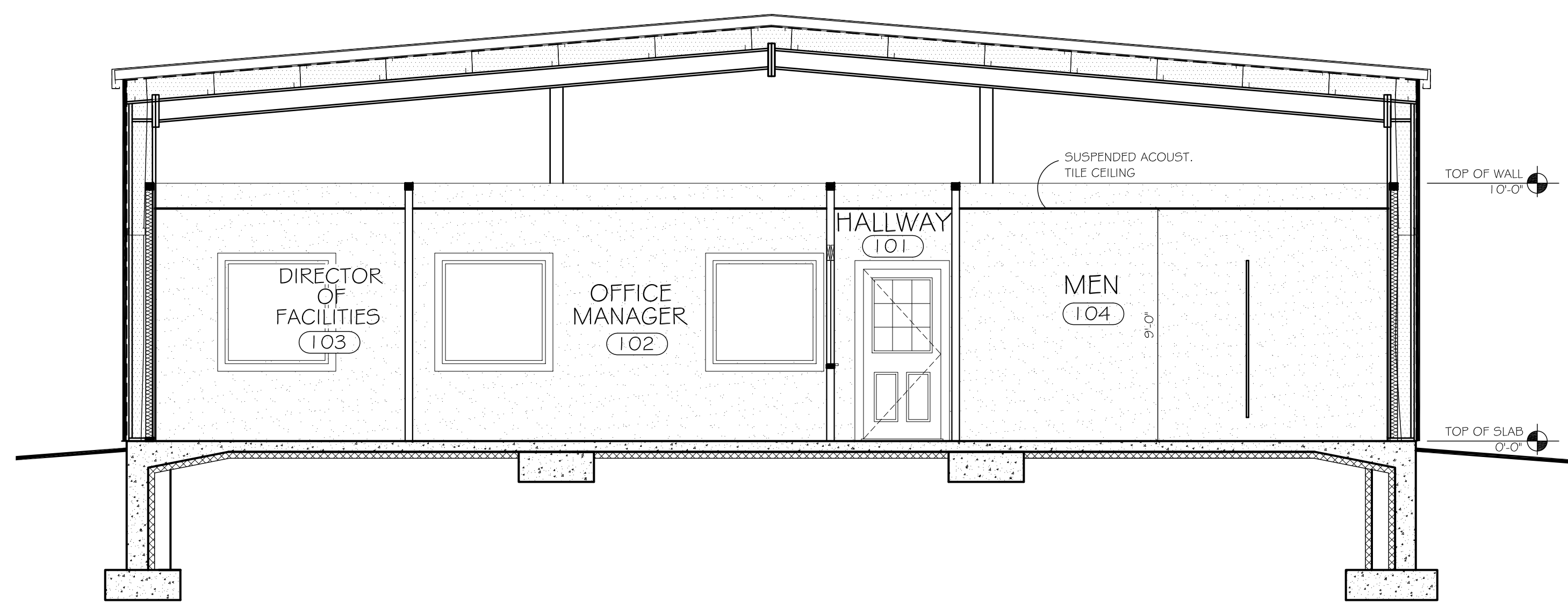
1 BUILDING SECTION "A" Scale: 1/4" = 1'-0"
