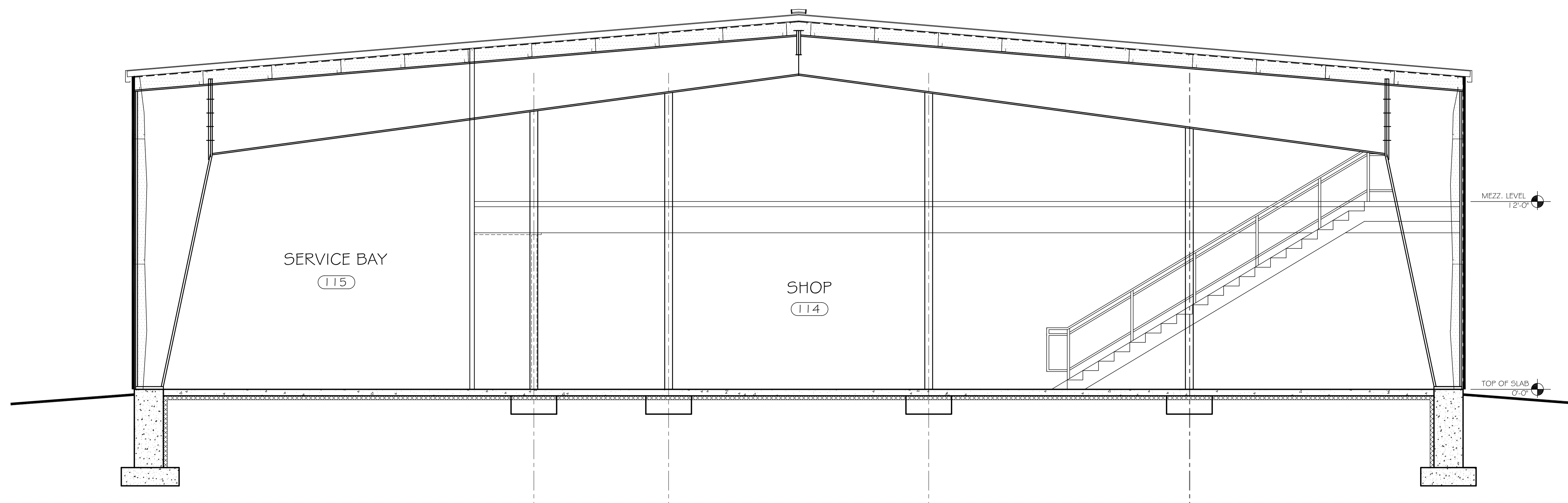
1 BUILDING SECTION "D" Scale: 1/4" = 1'-0"
