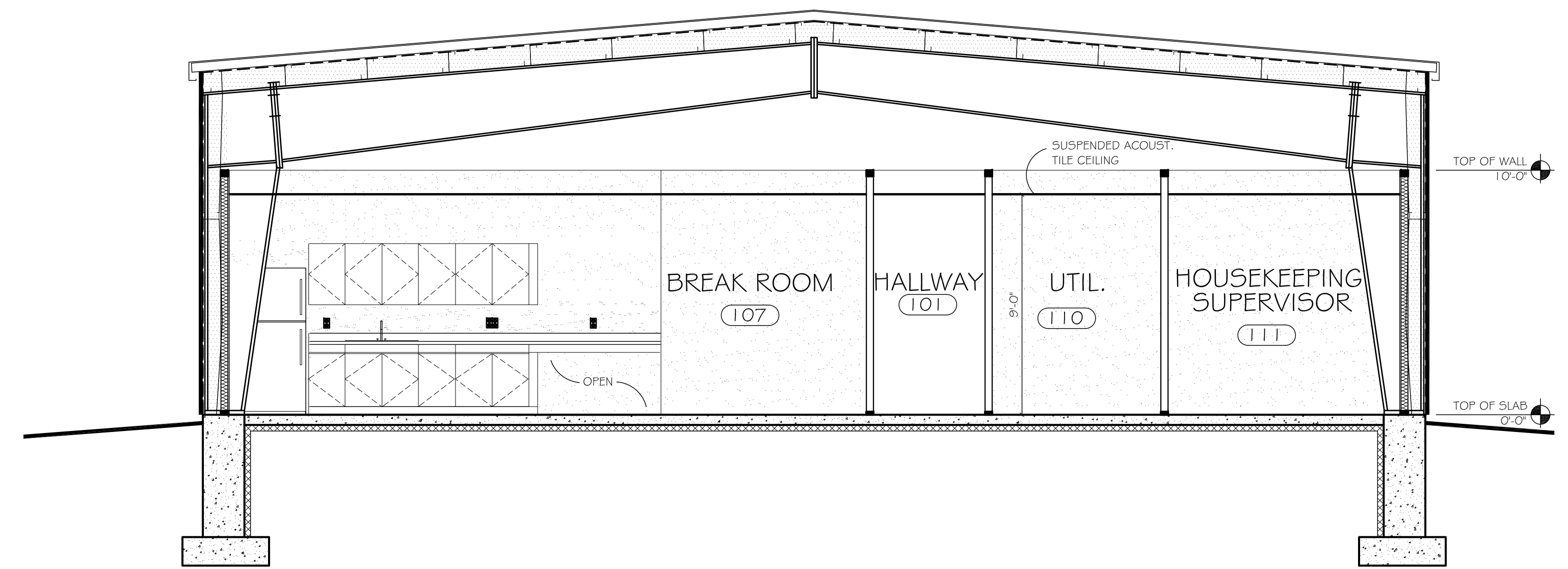
2 BUILDING SECTION "B" Scale: 1/4" = 1'-0"
