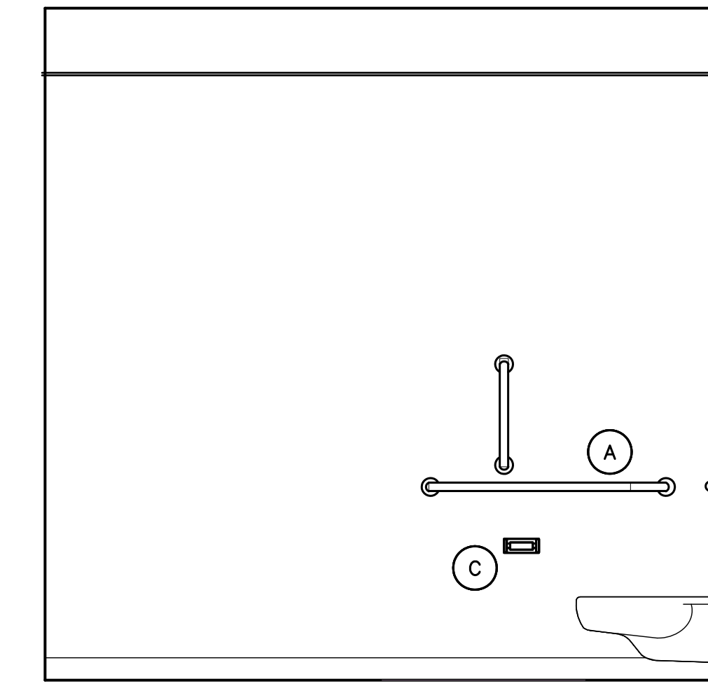
WALL "A"
